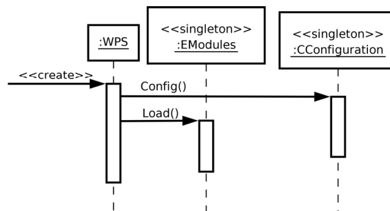
Figure 1: A UML diagram showing the Initialisation sequence.
