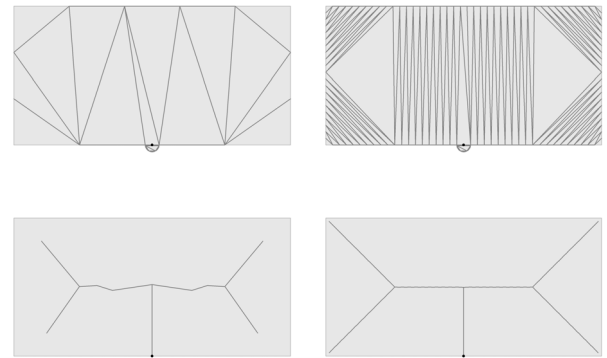
Fig. 7. Approximating the medial axis using Delaunay triangulation. Left: Boundary point density 5 m. Right: Boundary point density 0,5 m. Above: Triangles of Delaunay triangulation, Below: Resulting medial axis.
